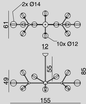
1574.12L.LIN LAMPADARIO / CHANDELIER Glass 12 x Ø 12-14 cm 12 x G9 33 W
