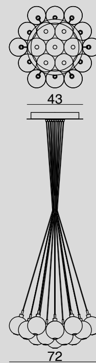
1292.19L SOSPENSIONE A PIASTRA / HANGING LAMP WITH CEILING PLATE Glass 19 x Ø 14 cm - Cable 250 cm 19 x G9 33 W
