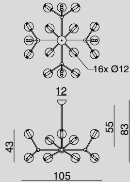
1574.12.4.16L LAMPADARIO / CHANDELIER Glass 16 x Ø 12 cm 16 x G9 33 W
