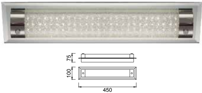
5533 Cromo-Chrome LED 13W 4000K 1100lm
