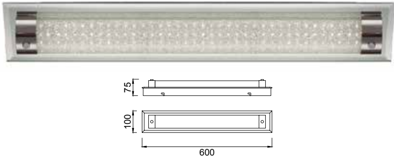
5532 Cromo-Chrome LED 21W 4000K 1800lm
